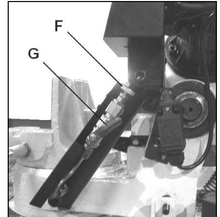
Fig 9...MBS-708CS
